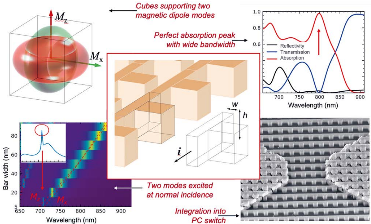
Figure 4. Perfectly-absorbing network of PC resonators. The metasurface consists of an array of cubes connected by side bars into a network (center). Each cube supports magnetic dipole modes (top left) and the bar allows excitation of the dark mode M_z . Perfect absorption occurs if the modes are degenerate (top right); the modes are tuned by adjusting the cube or the bar geometry (bottom left, from Ref. 13). The metasurface serves as the PC channel (bottom right).
