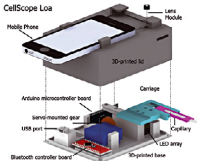
A schematic of the CellScope Loa device, a mobile phone-based video microscope. The device includes a 3D-printed case housing simple optics, circuitry and controllers to help process the sample of blood. CellScope Loa can quantify levels of the Loa bus parasitic worm directly from whole blood in less than 3 minutes. (Image by Mike D'Ambrosio and Matt Bakalar, Fletcher Lab, UC Berkeley)
