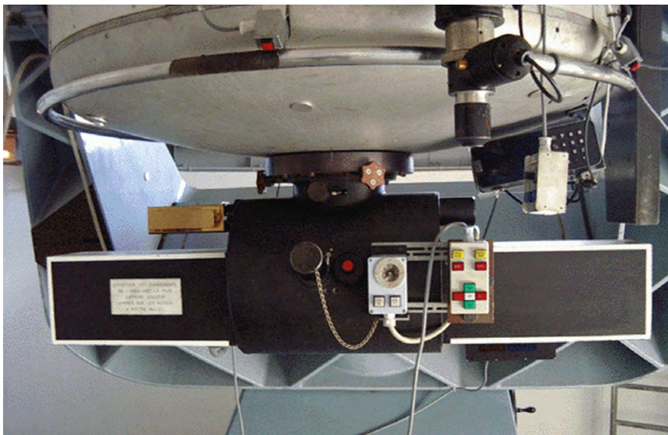
Figure 2. CORAVEL attached at the Cassegrain focus of the 1 m Swiss telescope at OHP.
