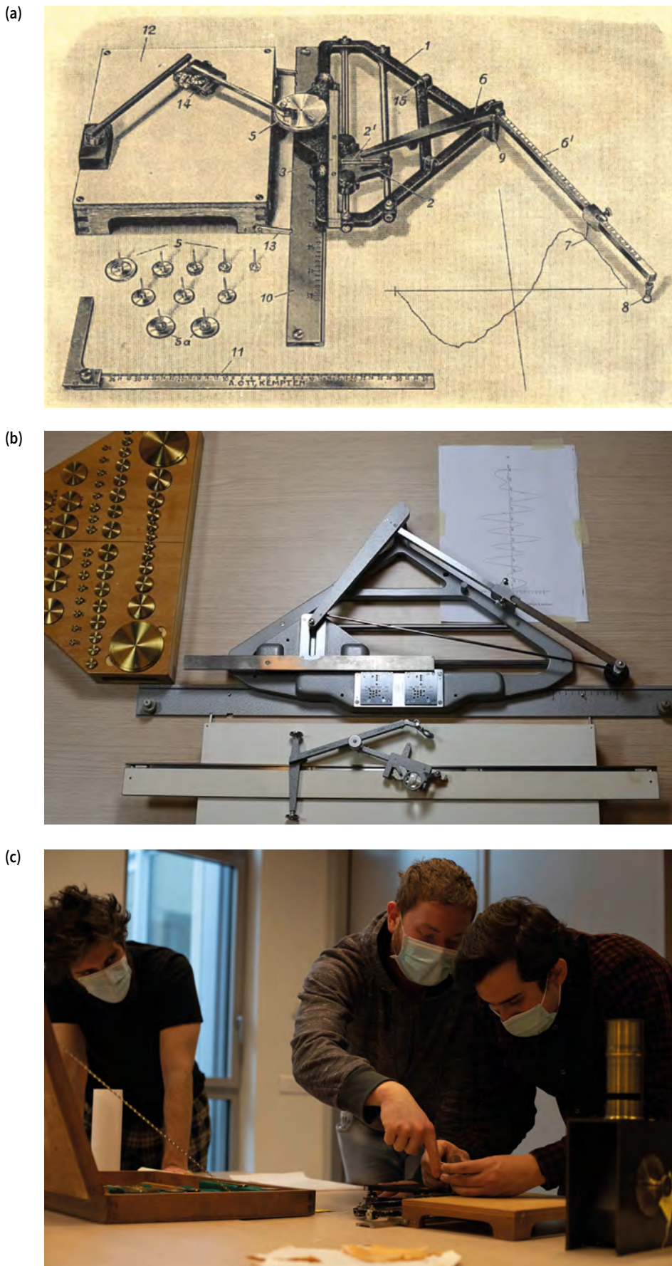
Figure 3. The Mader-Ott Harmonic Analyser used from 1909 to 1960. a) Illustration of how the harmonic analyzer works. b) Mader-Ott Harmonic Analyser from Optics department lab collection, FEMTO-ST Institute, Besançon. c) Master students from graduate school EIPHI during labwork with the harmonic analyzer.
