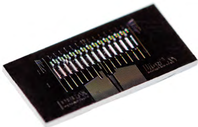
Label-free biosensor PIC of Delta Diagnostics for biomolecular interaction analysis and protein quantitation. ©DeltaDiagnostics.
